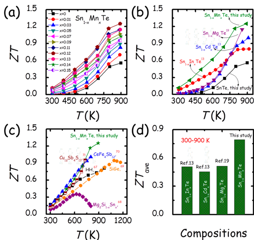
Figure 5. (a) Temperature-dependent ZT values for \text{Sn}_{1-x}\text{Mn}_x\text{Te} . (b) Comparison of the ZT values of several singly doped \text{SnTe} , 13,19 among which Mn-doped \text{SnTe} clearly has the highest performance in the entire temperature range because of the stronger valence band convergence by higher doping limit of Mn. (c) Comparison of temperature-variant ZT of Mn-doped \text{SnTe} with some other p-type lead-free systems including half-Heusler compound (HH), 67 \text{Mg}_2\text{Si}_{1-x}\text{Sn}_x , 68 \text{SiGe} alloy, 69 skutterudite ( \text{CeFe}_4\text{Sb}_{12} ), 70 and a representative of tetrahedrites ( \text{Cu}_{12}\text{Sb}_4\text{S}_{13} ). 71 (d) Comparison of average ZT ( ZT_{\text{ave}} ) in the temperature interval of 300–900 K of several singly doped p-type \text{SnTe} , 13,19 among which Mn-doped \text{SnTe} has a ZT_{\text{ave}} that outperforms any others.
